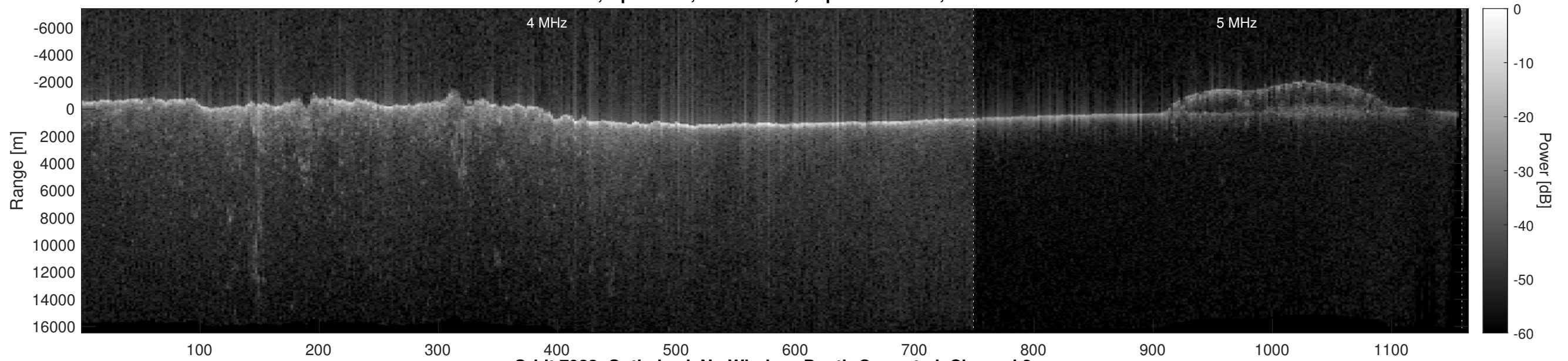
Orbit 7923, Optimized, No Window, Depth-Corrected, Channel 2
