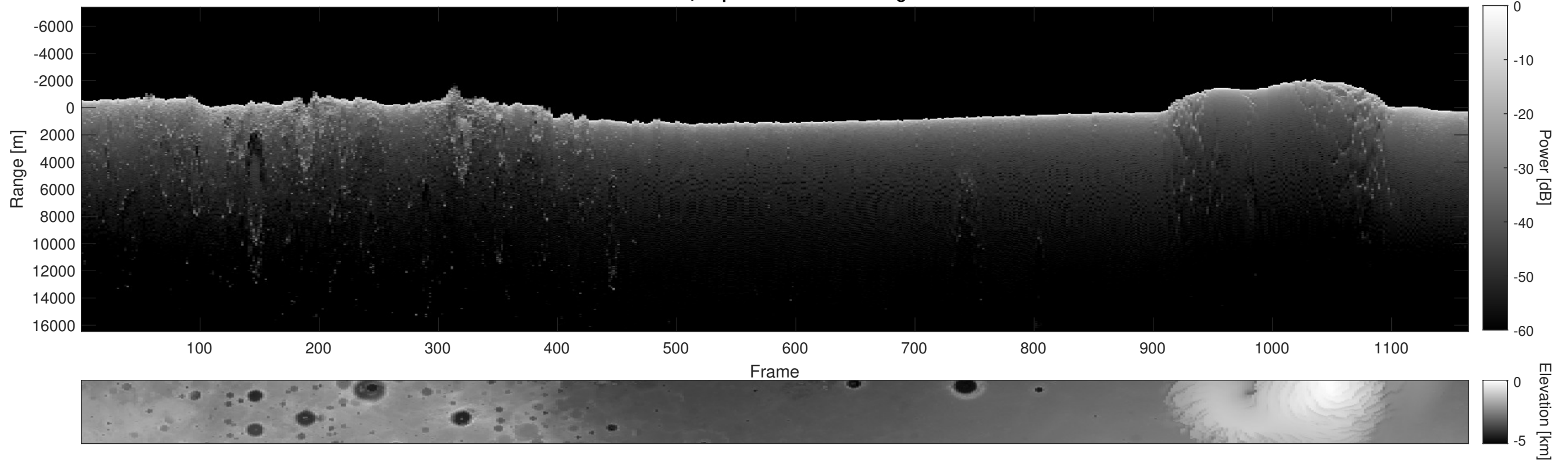
Orbit 7923, Depth-Corrected Cluttergram
