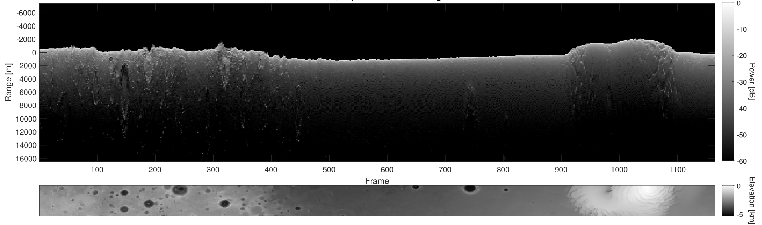
Orbit 7923, Depth-Corrected Cluttergram
