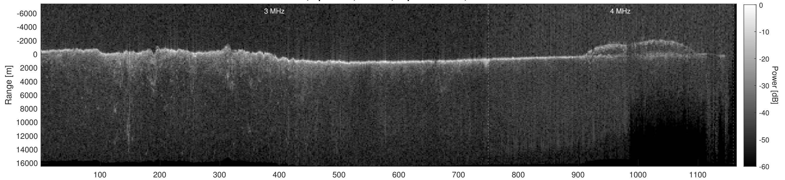
Orbit 7923, Depth-Corrected Cluttergram
