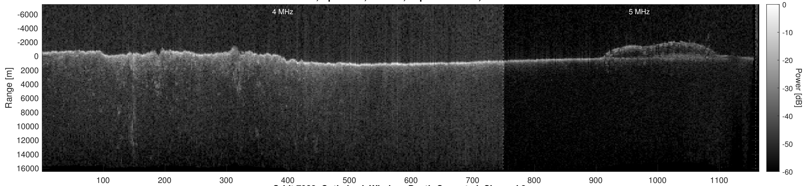
Orbit 7923, Optimized, Window, Depth-Corrected, Channel 2
