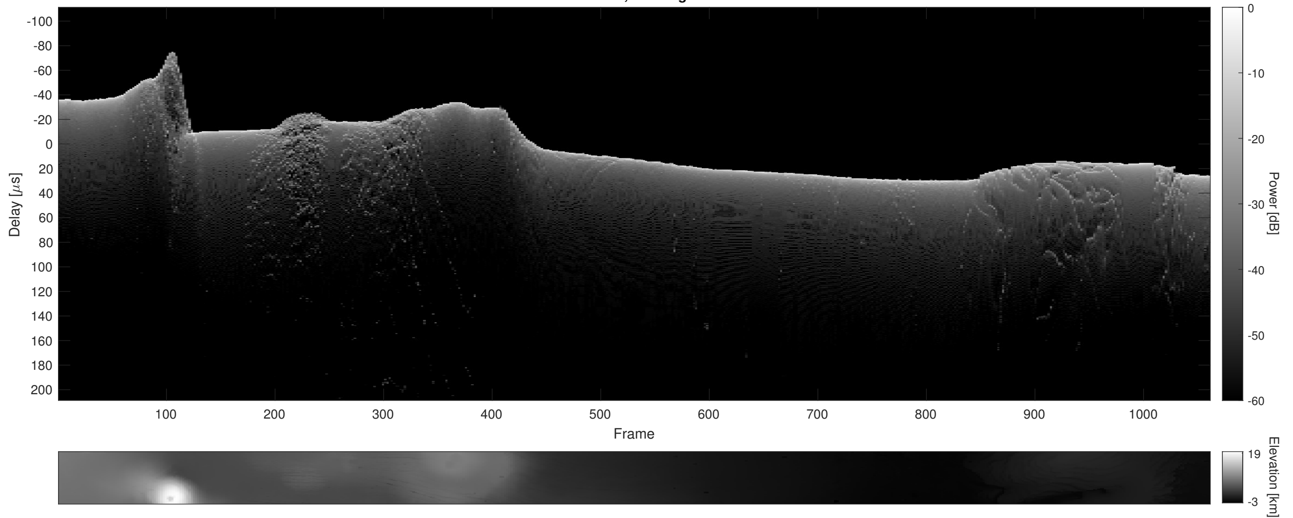
Orbit 7924, Cluttergram
