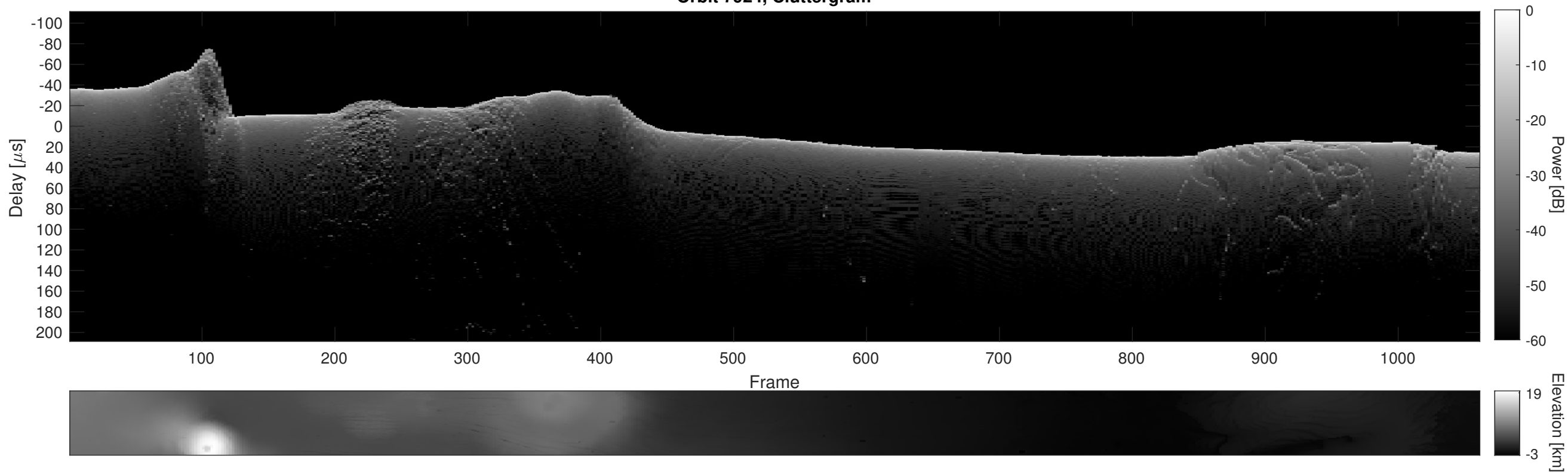
Orbit 7924, Cluttergram
