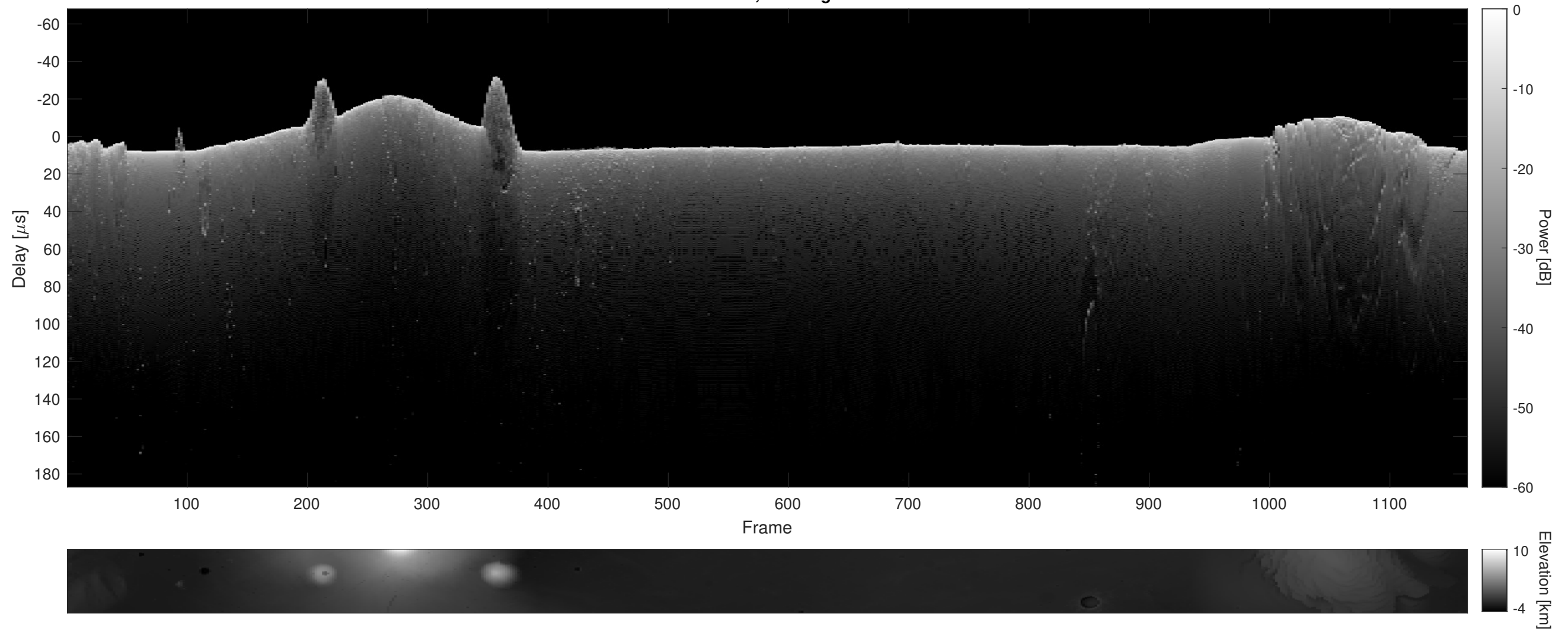
Orbit 7925, Cluttergram
