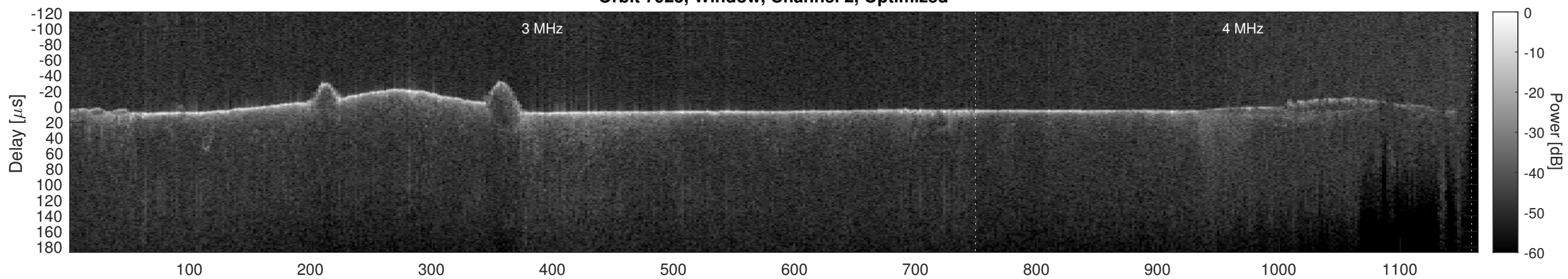
Orbit 7925, Cluttergram
