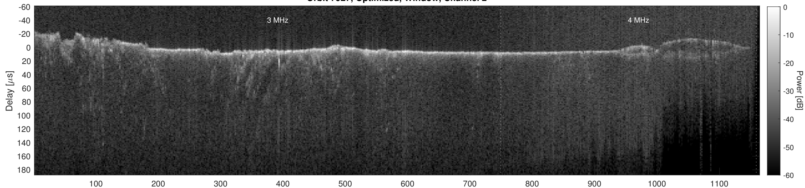
Orbit 7927, Cluttergram
