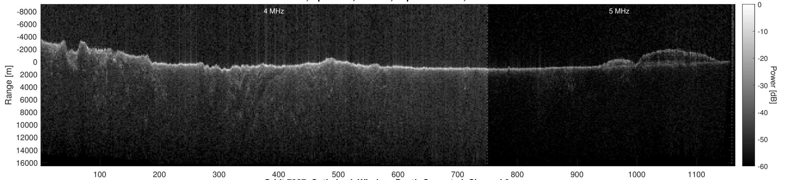
Orbit 7927, Optimized, Window, Depth-Corrected, Channel 2
