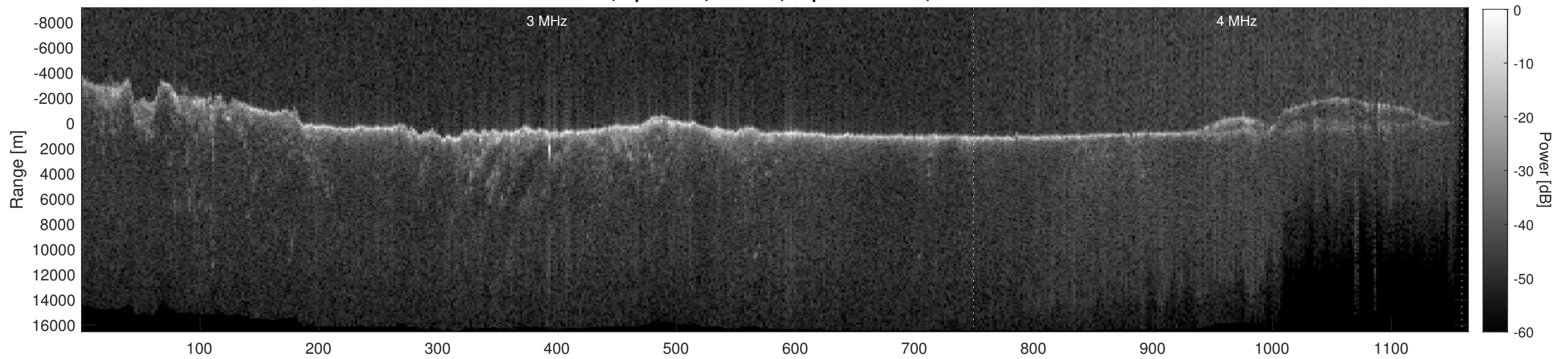
Orbit 7927, Depth-Corrected Cluttergram
