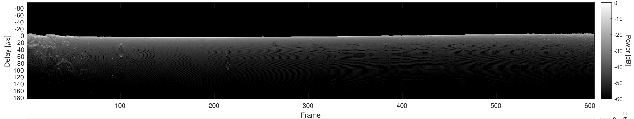
Orbit 7928, Cluttergram
