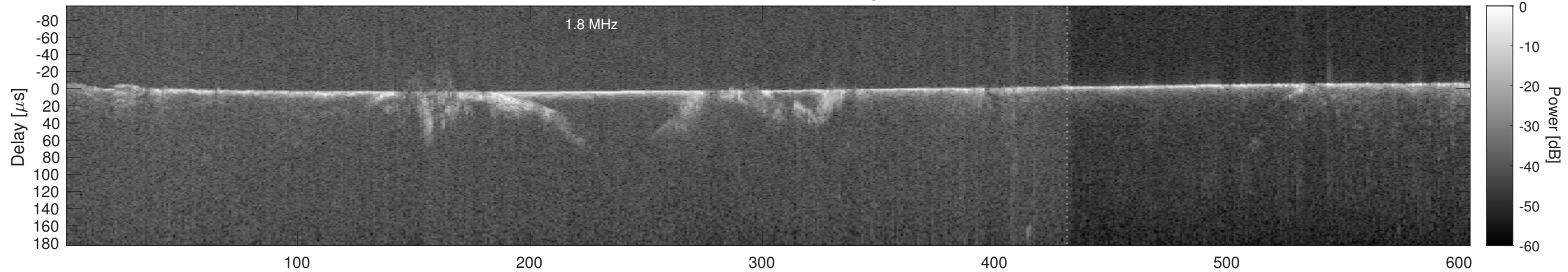
Orbit 7928, Cluttergram
