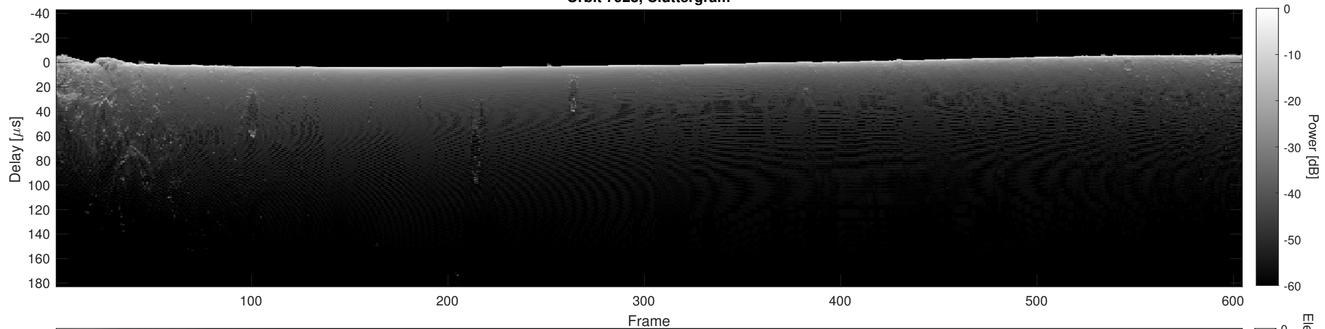
Orbit 7928, Cluttergram
