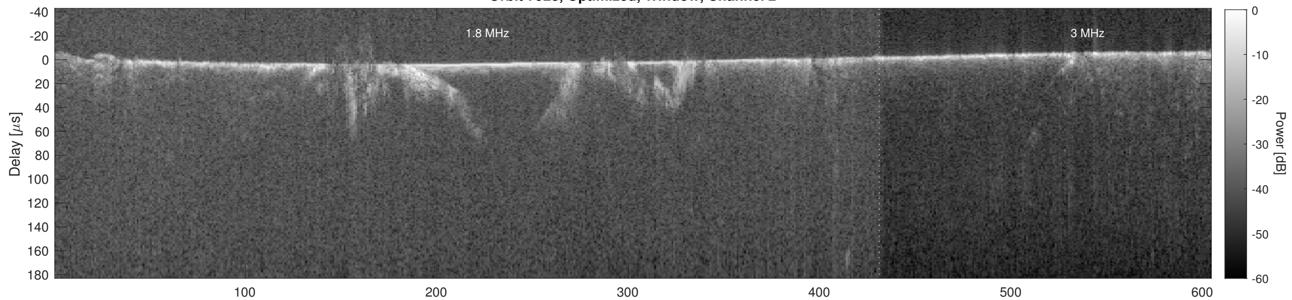
Orbit 7928, Cluttergram
