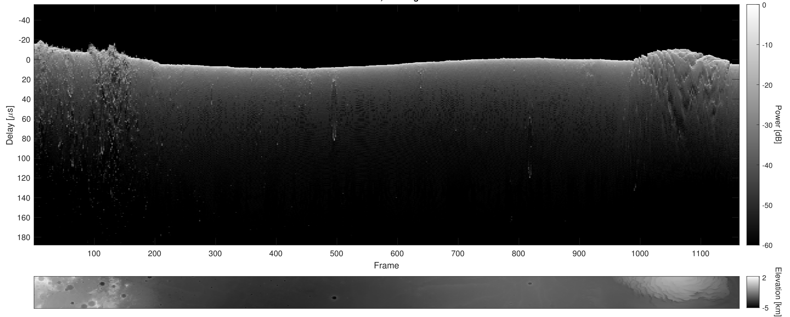
Orbit 7929, Cluttergram
