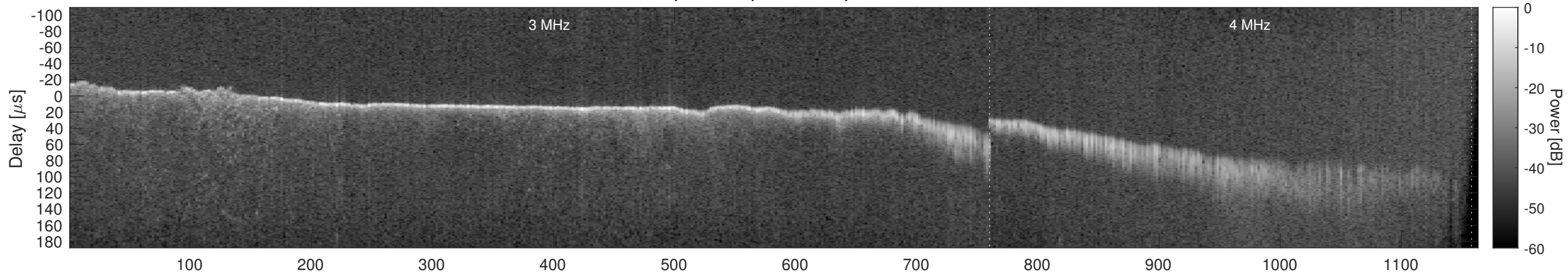
Orbit 7929, Window, Channel 2, Chapman
