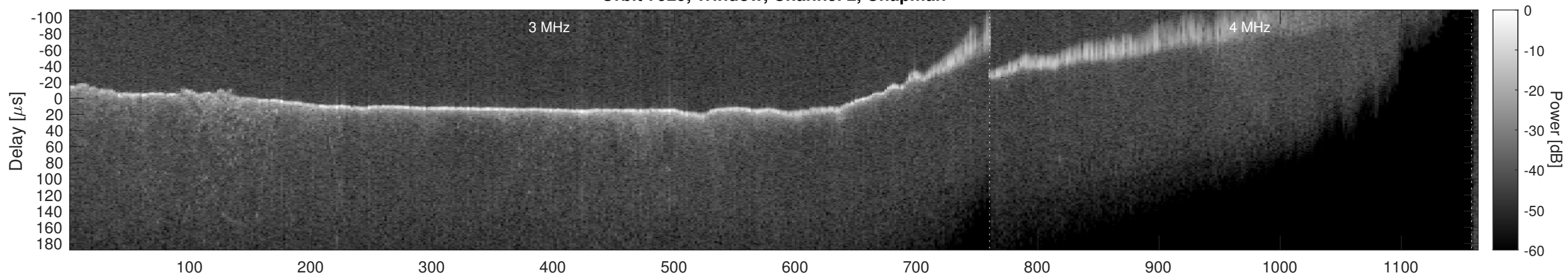
Orbit 7929, Window, Channel 2, Optimized
