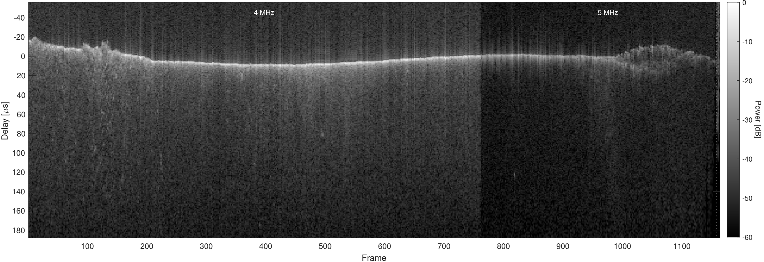
Orbit 7929, Optimized, No Window, Channel 2
