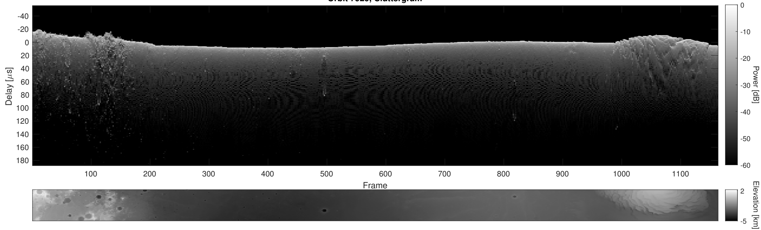
Orbit 7929, Cluttergram
