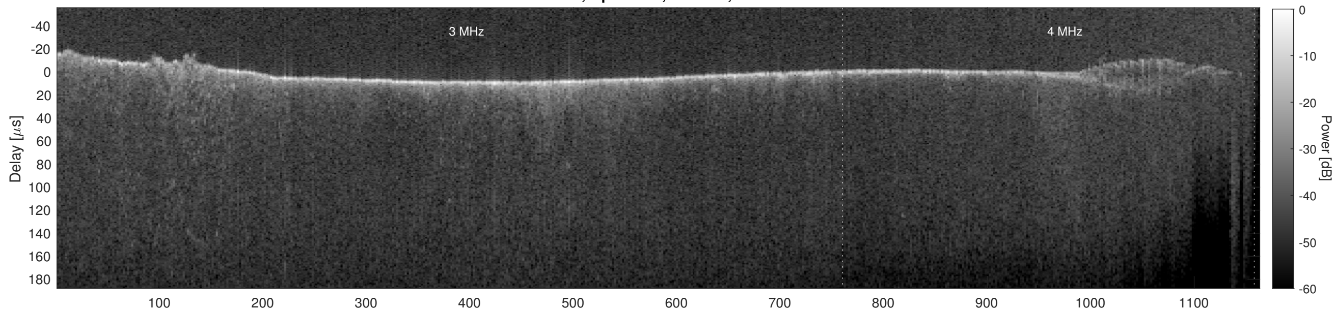
Orbit 7929, Cluttergram
