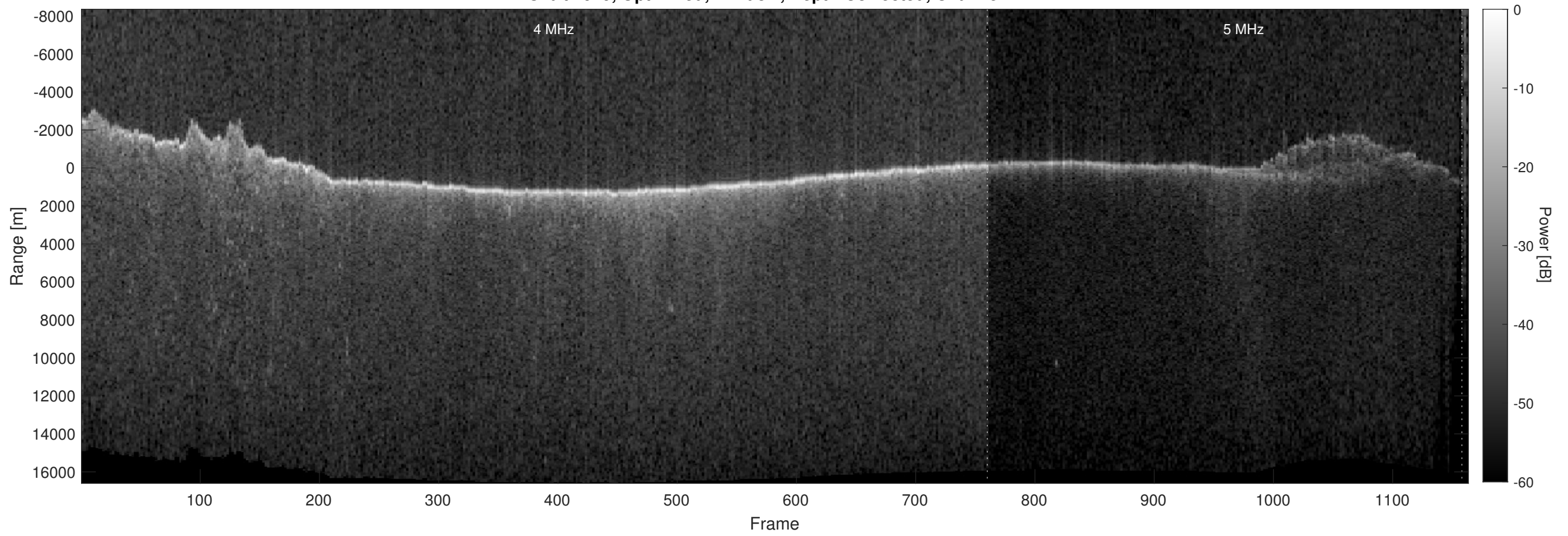
Orbit 7929, Optimized, Window, Depth-Corrected, Channel 2
