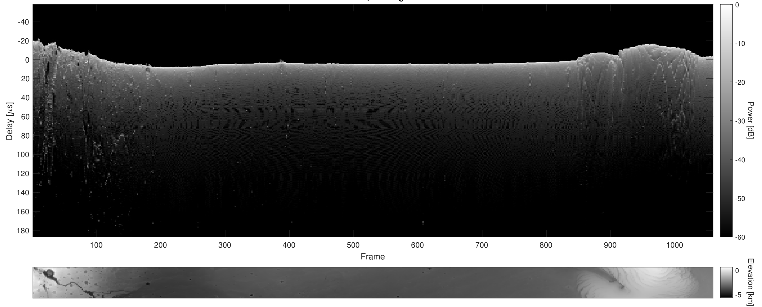
Orbit 7934, Cluttergram
