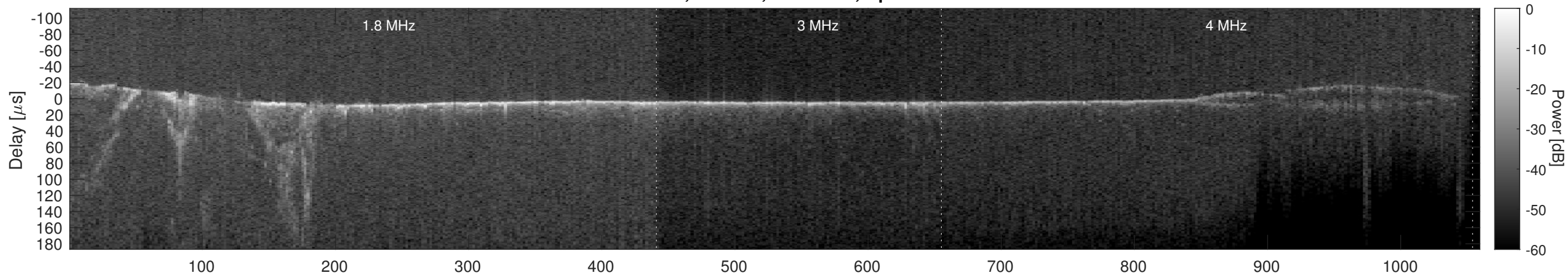
Orbit 7934, Cluttergram
