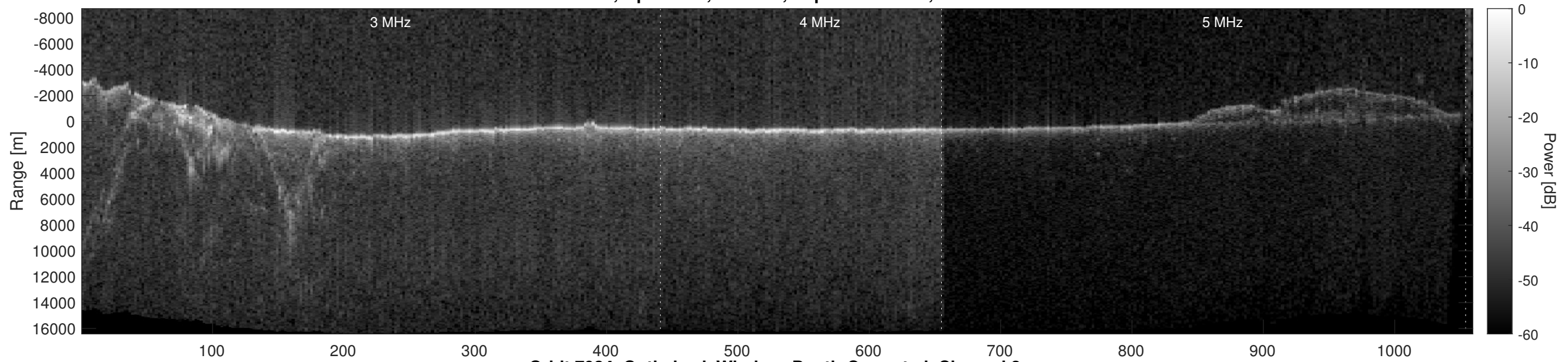
Orbit 7934, Optimized, Window, Depth-Corrected, Channel 2
