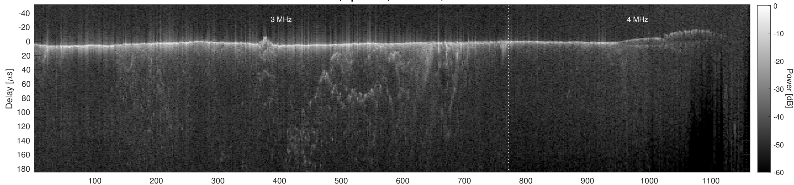
Orbit 7939, Cluttergram
