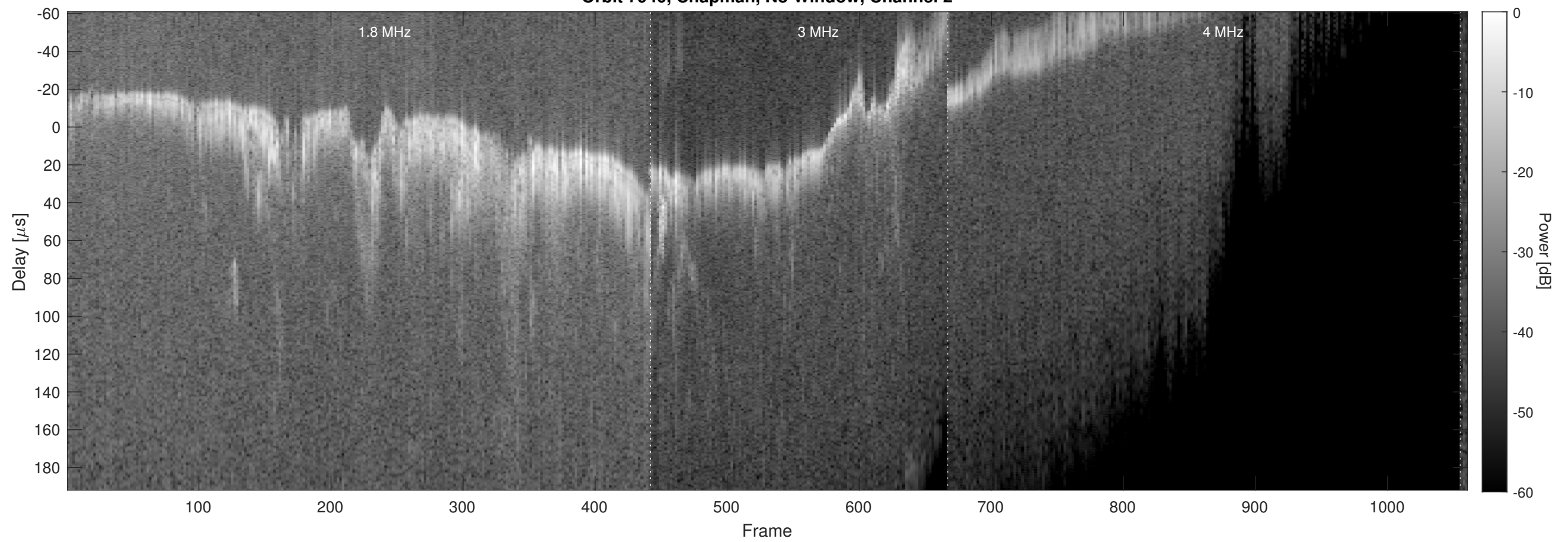
Orbit 7940, Chapman, No Window, Channel 2
