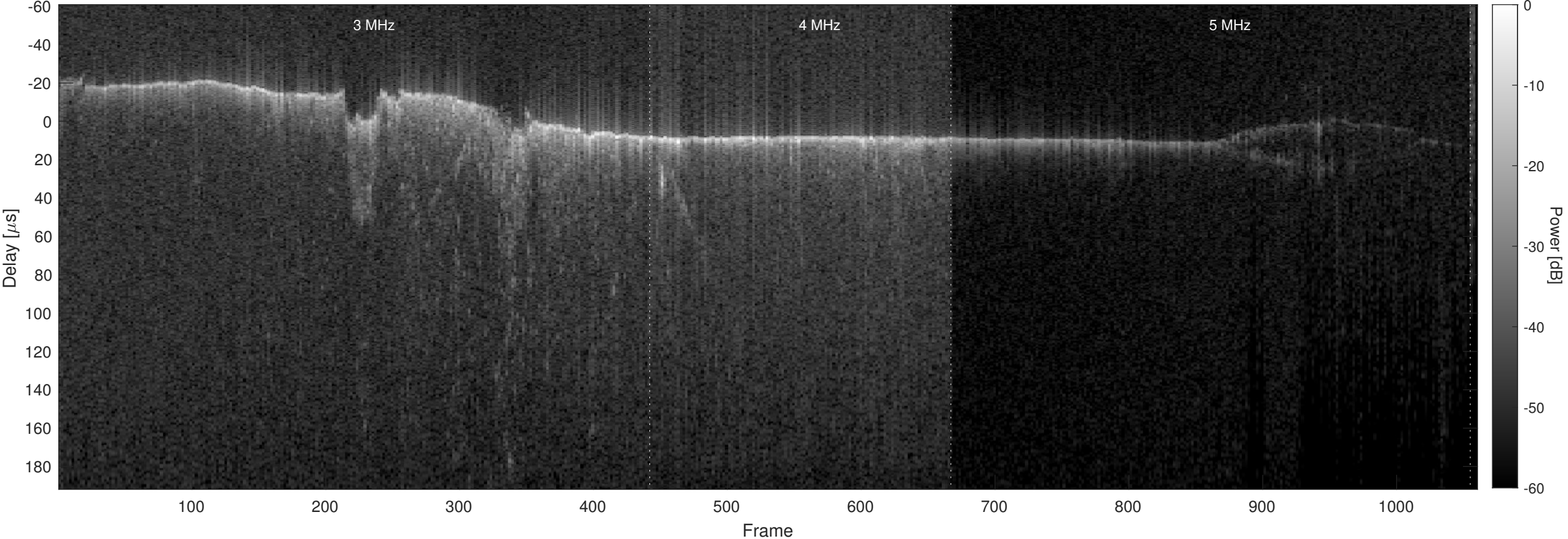
Orbit 7940, Optimized, No Window, Channel 2
