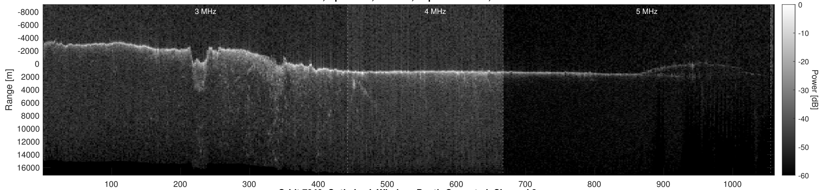
Orbit 7940, Optimized, Window, Depth-Corrected, Channel 2
