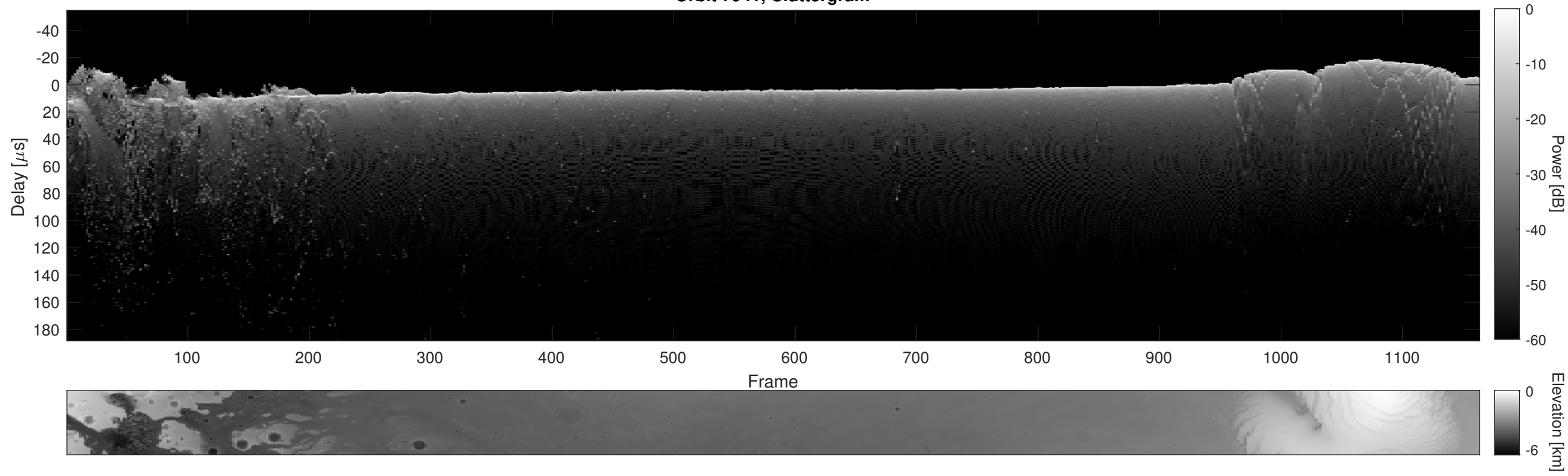
Orbit 7941, Cluttergram
