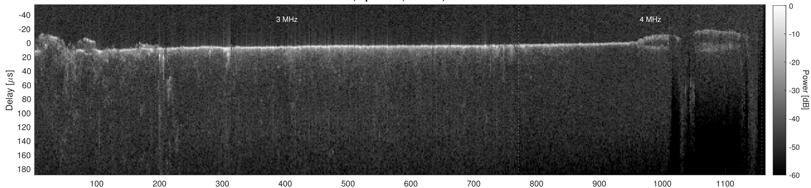
Orbit 7941, Cluttergram
