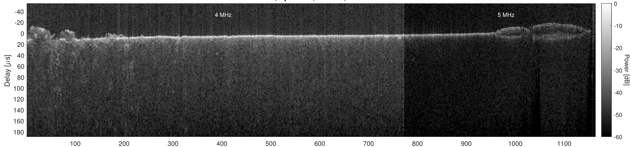
Orbit 7941, Optimized, Window, Channel 2
