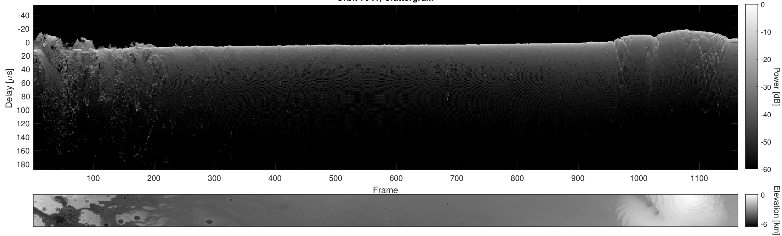
Orbit 7941, Cluttergram
