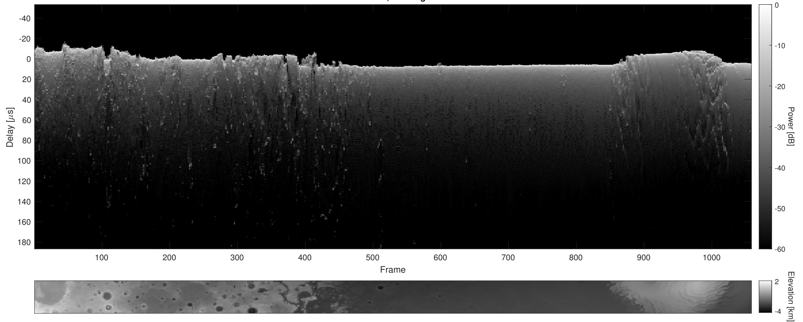
Orbit 7944, Cluttergram
