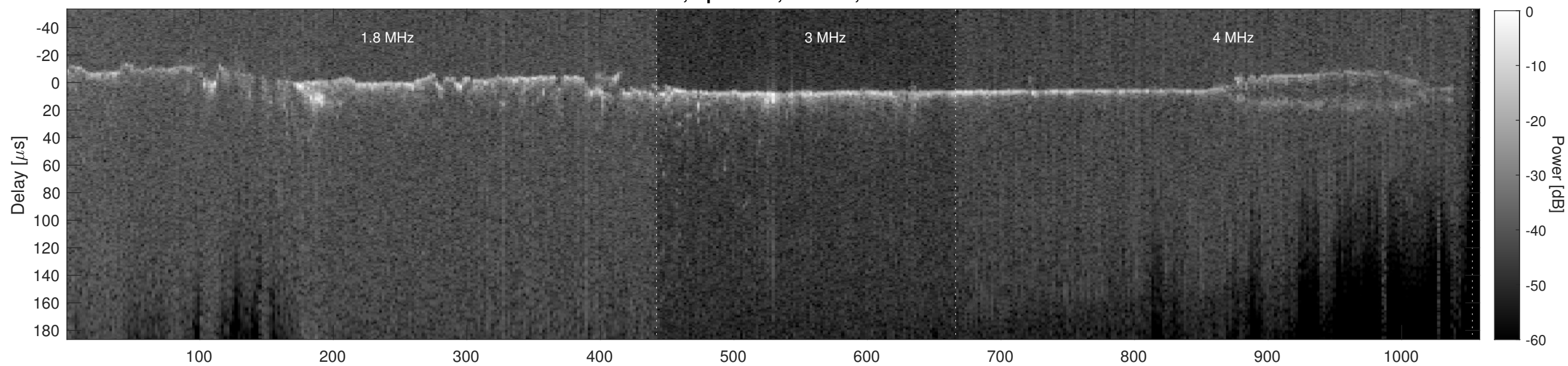
Orbit 7944, Cluttergram
