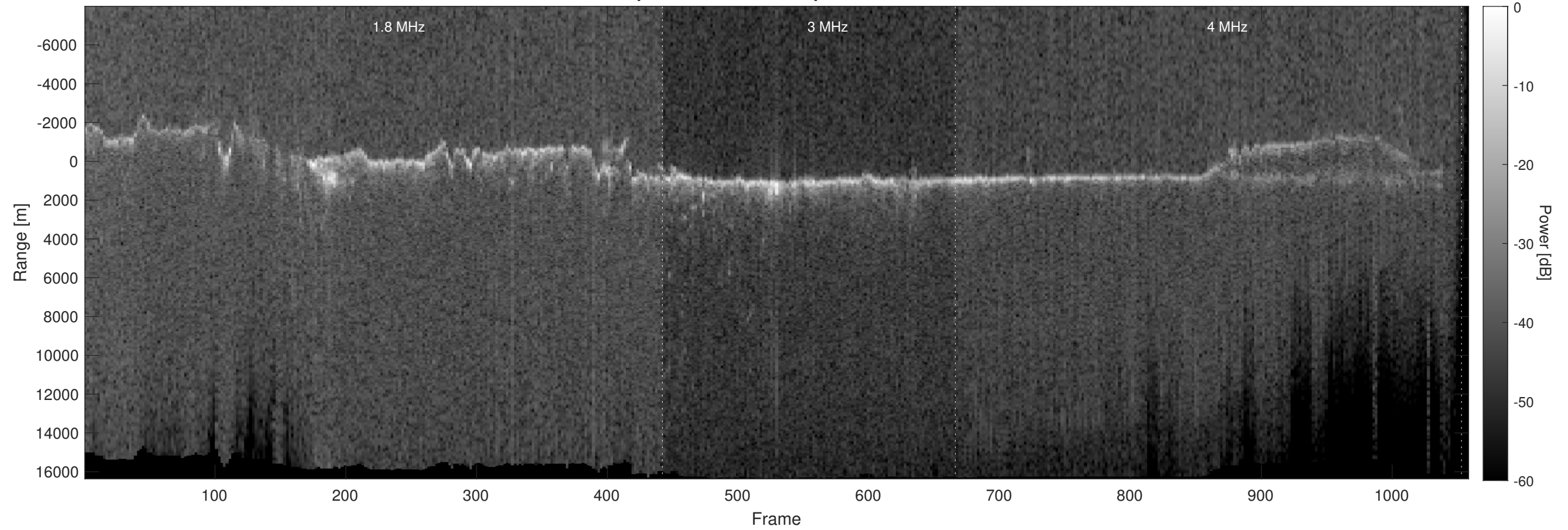
Orbit 7944, Optimized, Window, Depth-Corrected, Channel 2
