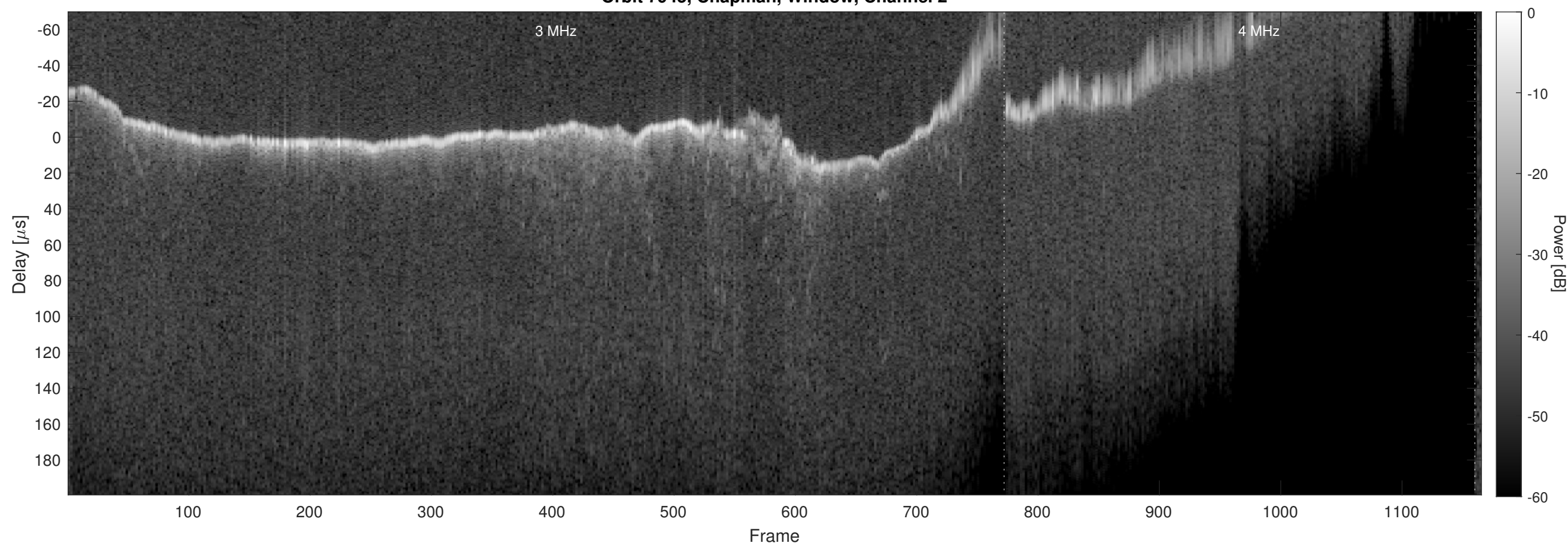
Orbit 7945, Chapman, Window, Channel 2
