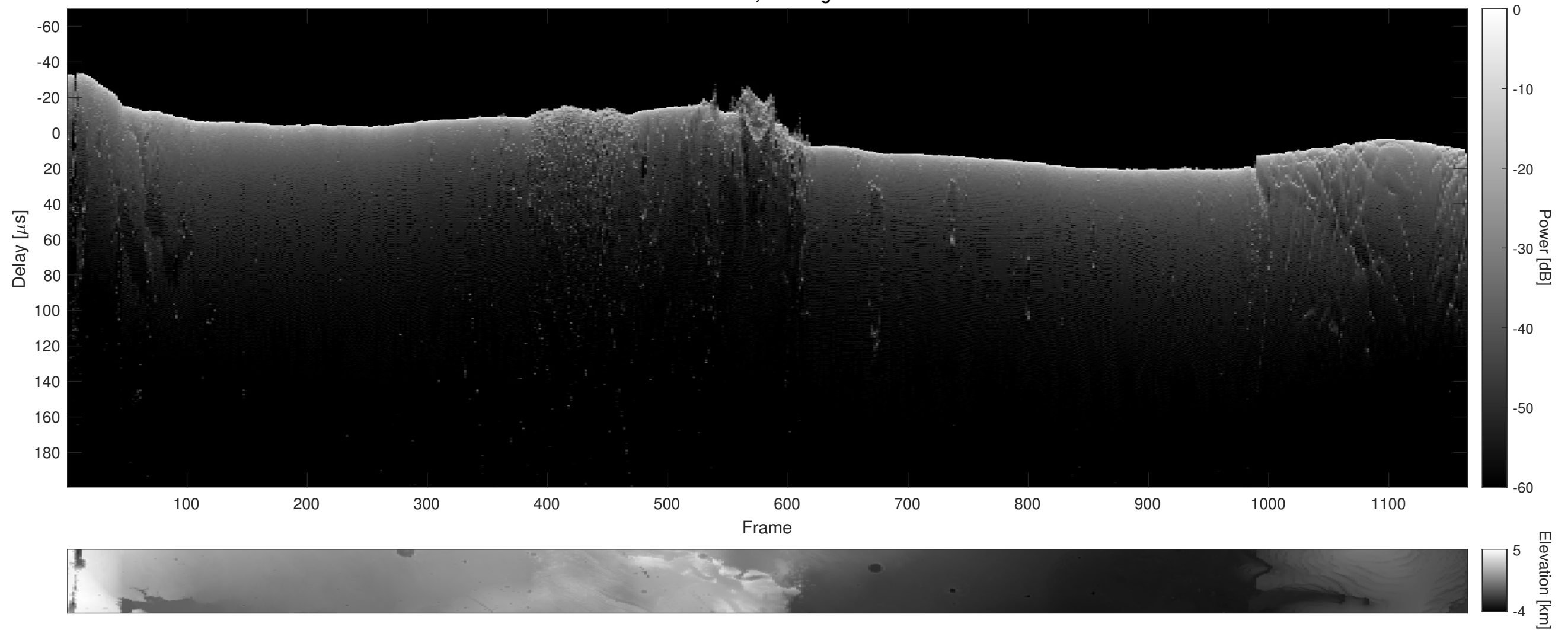
Orbit 7945, Cluttergram
