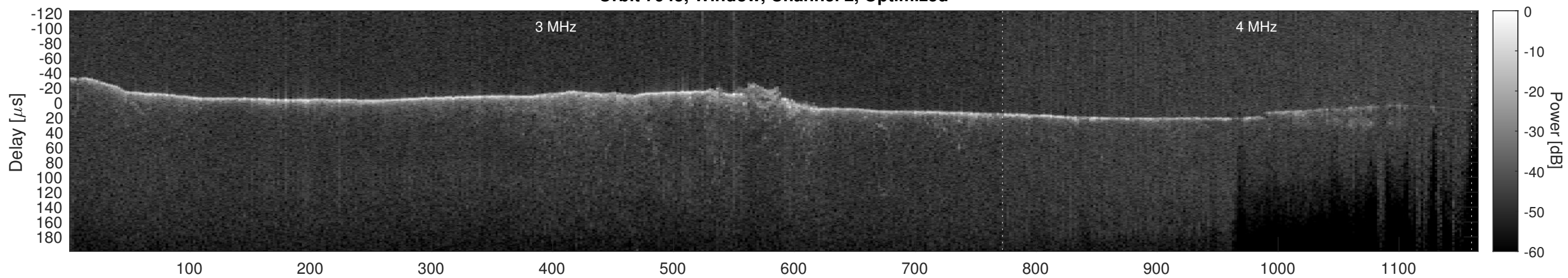
Orbit 7945, Cluttergram
