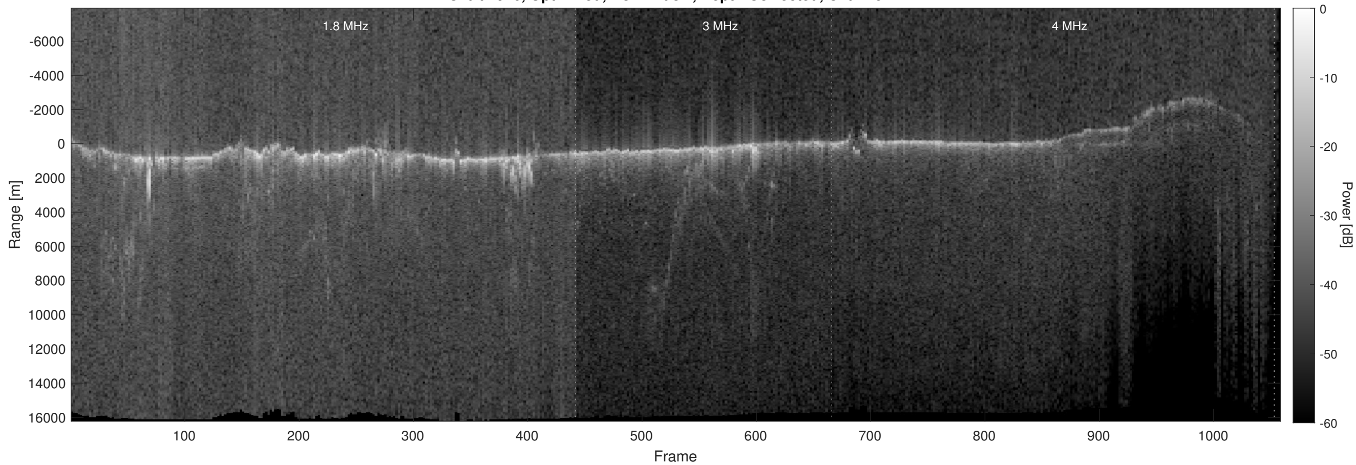
Orbit 7946, Optimized, No Window, Depth-Corrected, Channel 2
