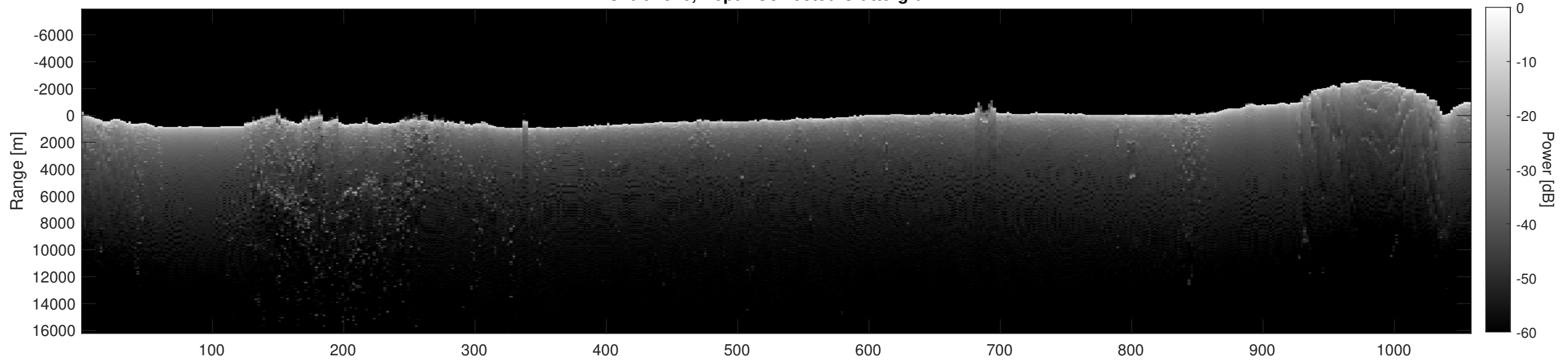
Orbit 7946, Depth-Corrected Cluttergram
