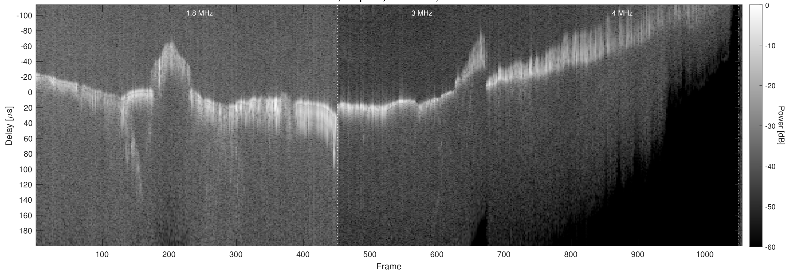
Orbit 7949, Chapman, No Window, Channel 2
