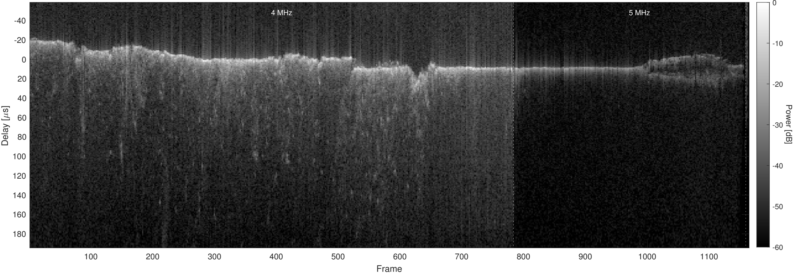
Orbit 7951, Optimized, No Window, Channel 2
