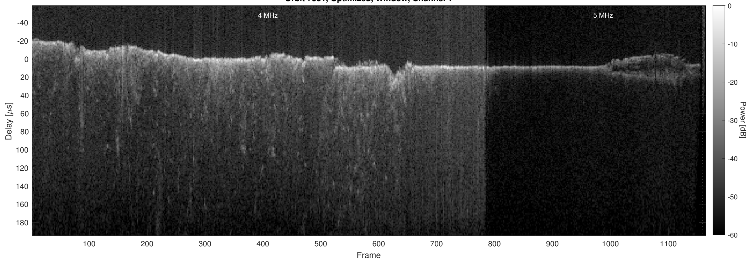
Orbit 7951, Optimized, Window, Channel 2
