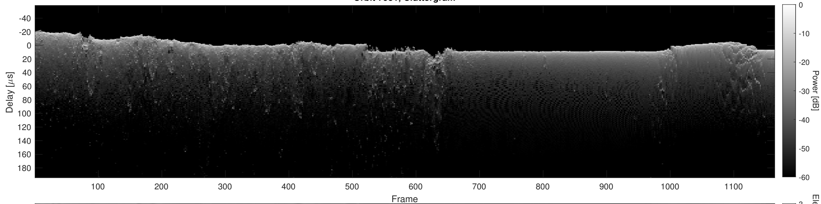
Orbit 7951, Cluttergram
