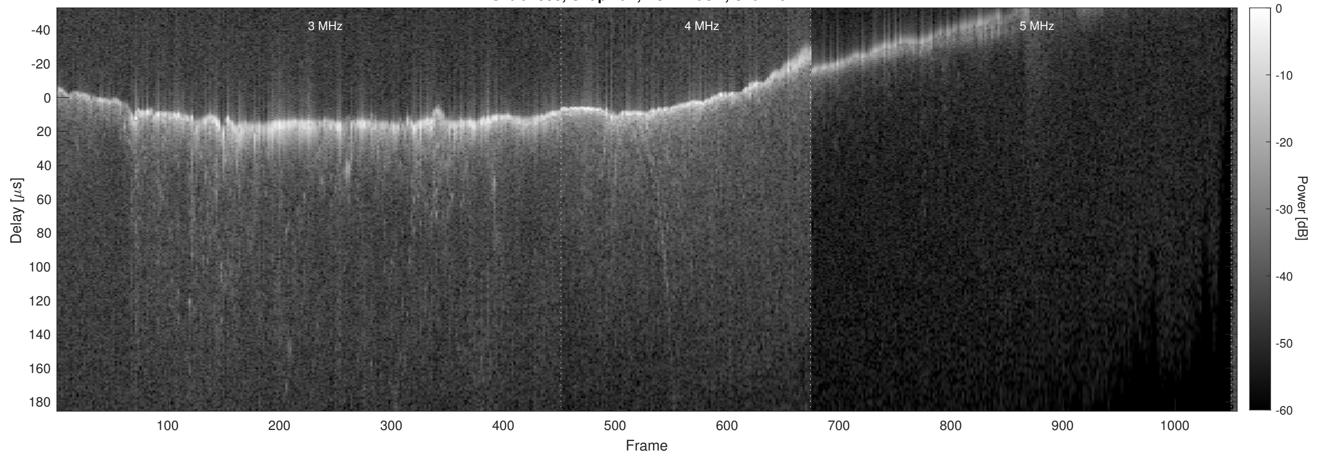
Orbit 7953, Chapman, No Window, Channel 2
