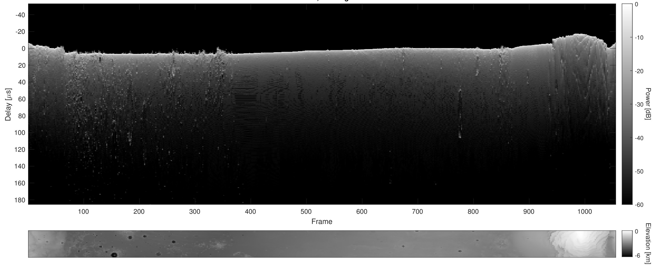
Orbit 7953, Cluttergram
