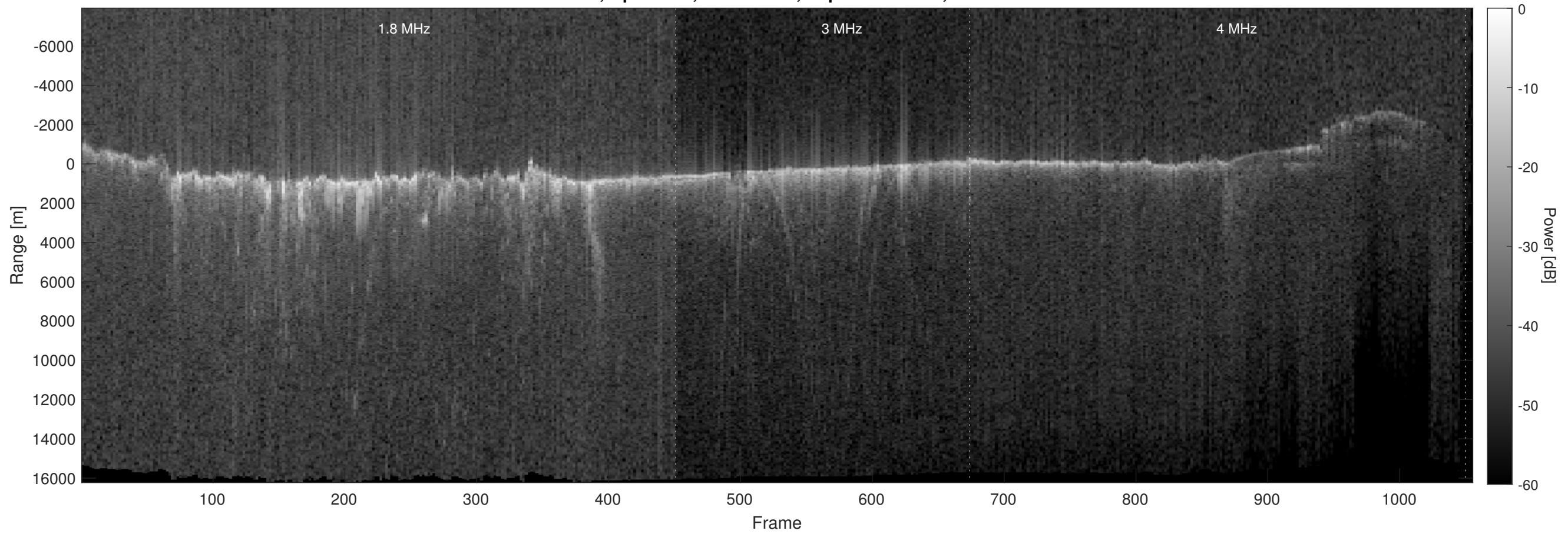
Orbit 7953, Optimized, No Window, Depth-Corrected, Channel 2
