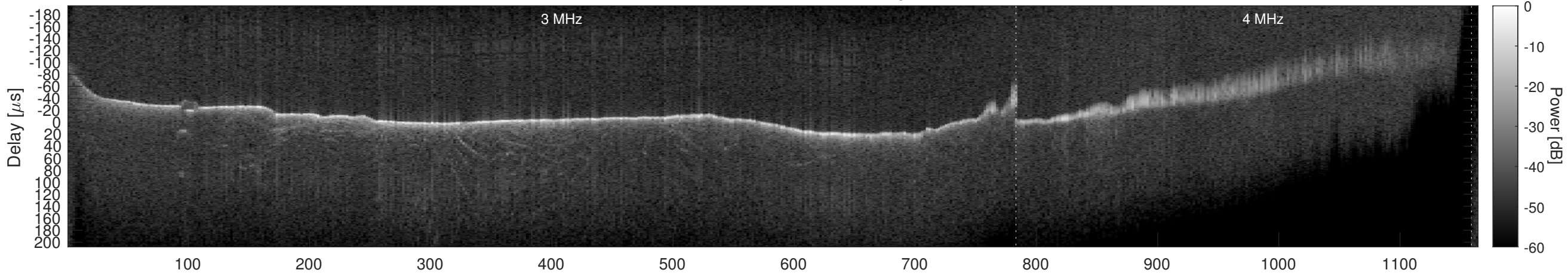
Orbit 7956, Window, Channel 2, Optimized
