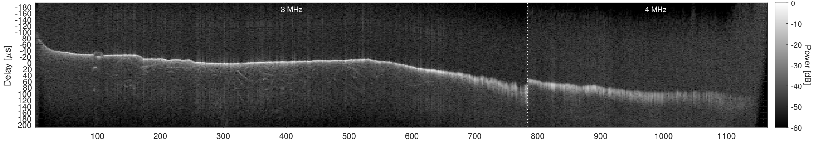
Orbit 7956, Window, Channel 2, Chapman
