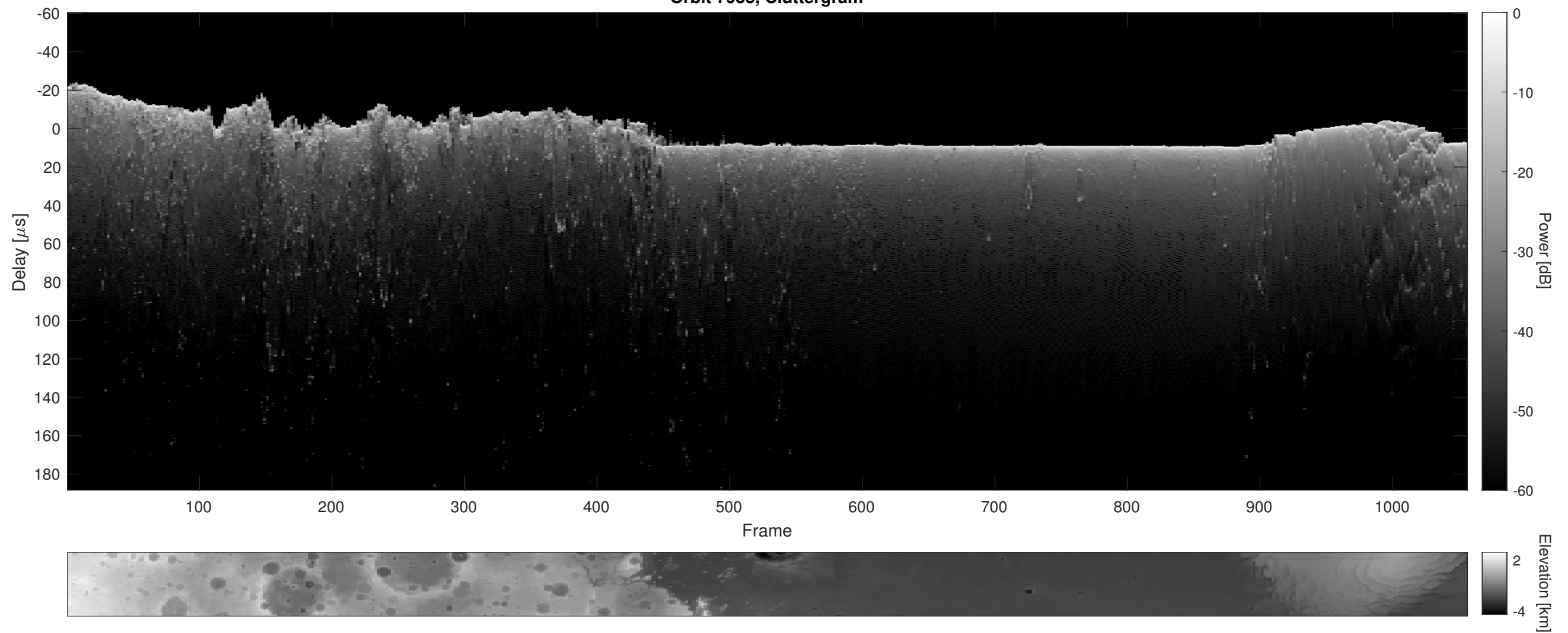
Orbit 7958, Cluttergram
