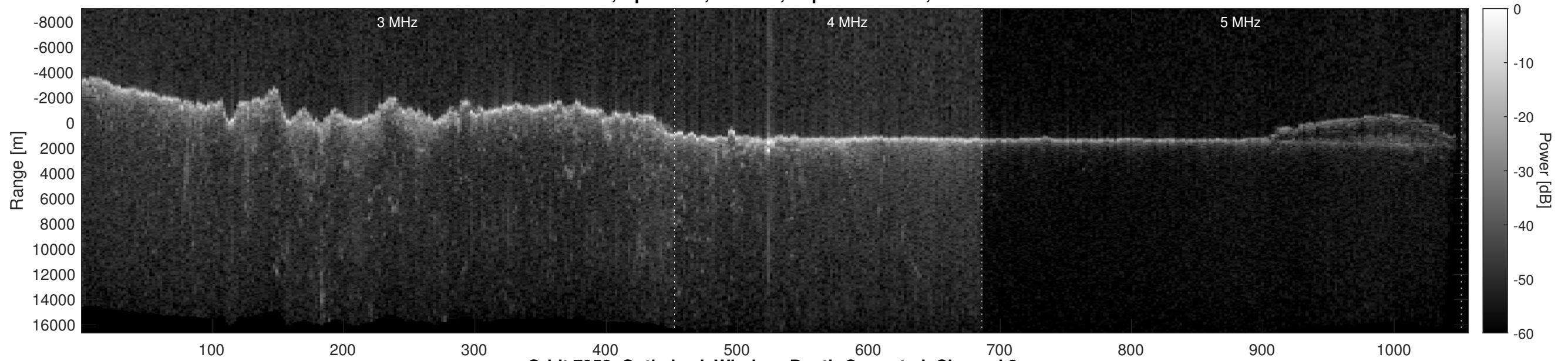
Orbit 7958, Optimized, Window, Depth-Corrected, Channel 2
