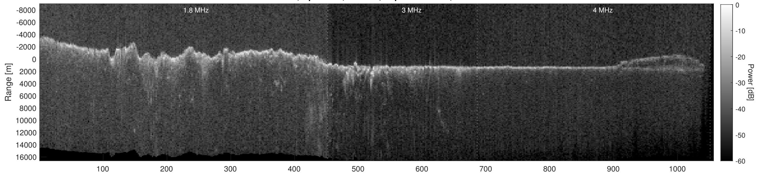
Orbit 7958, Depth-Corrected Cluttergram
