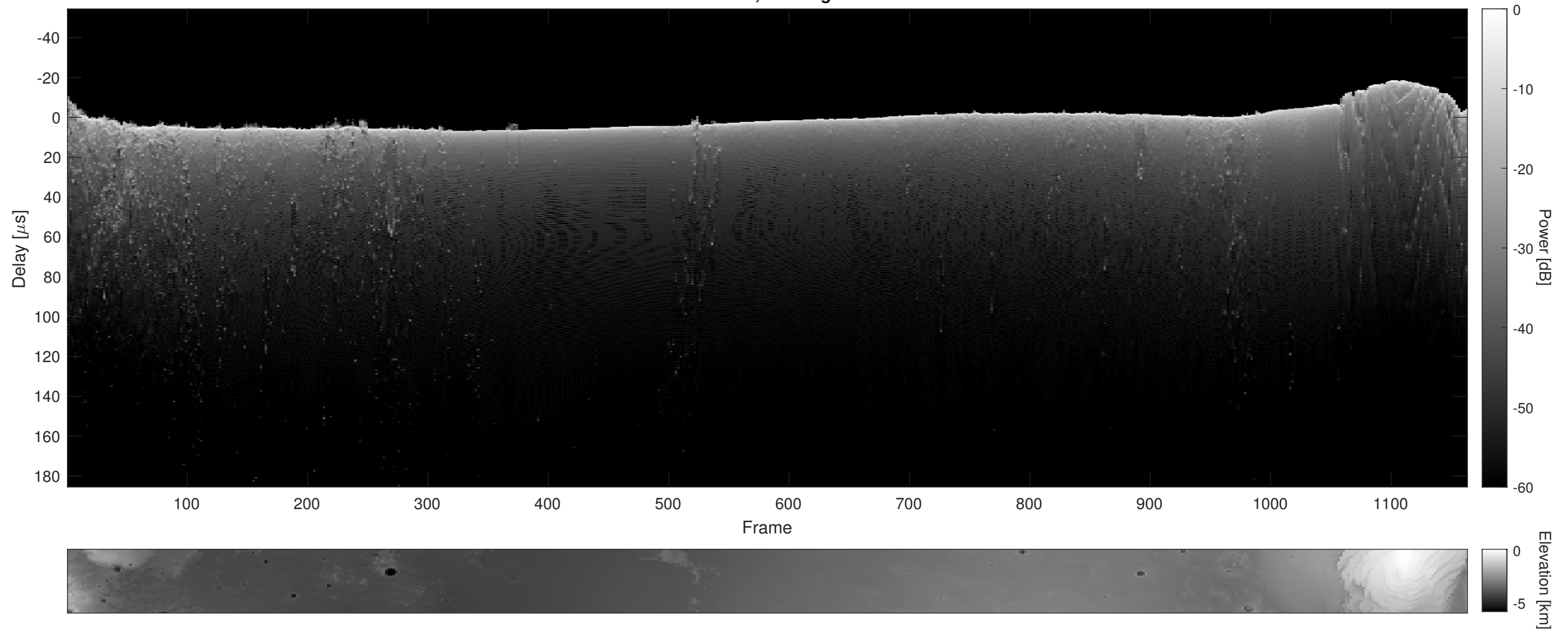
Orbit 7960, Cluttergram
