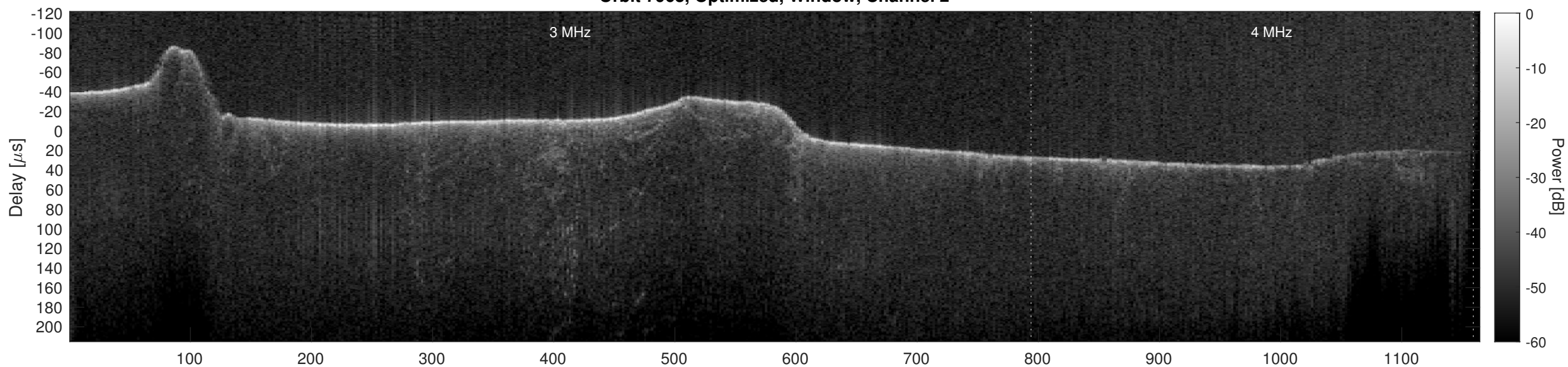
Orbit 7963, Cluttergram
