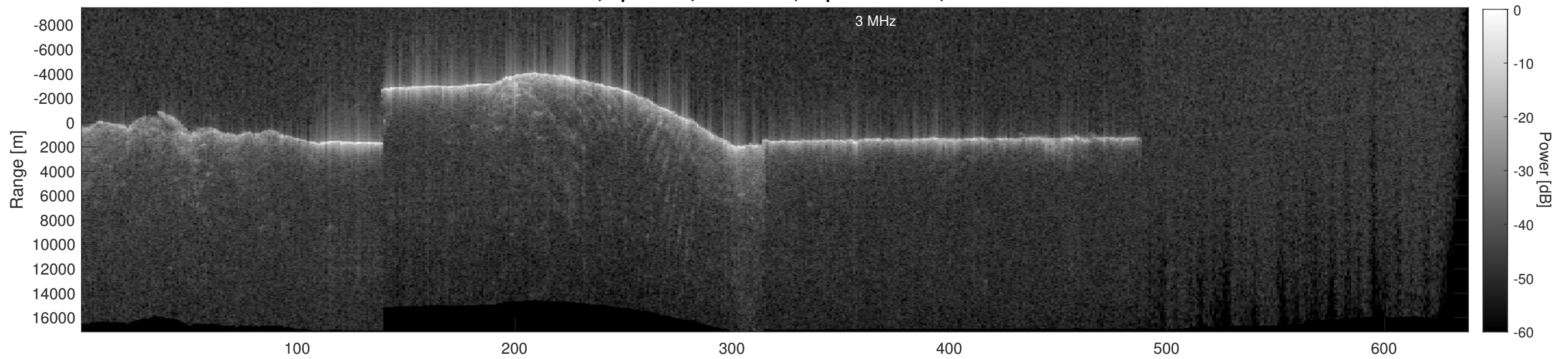
Orbit 7964, Depth-Corrected Cluttergram
