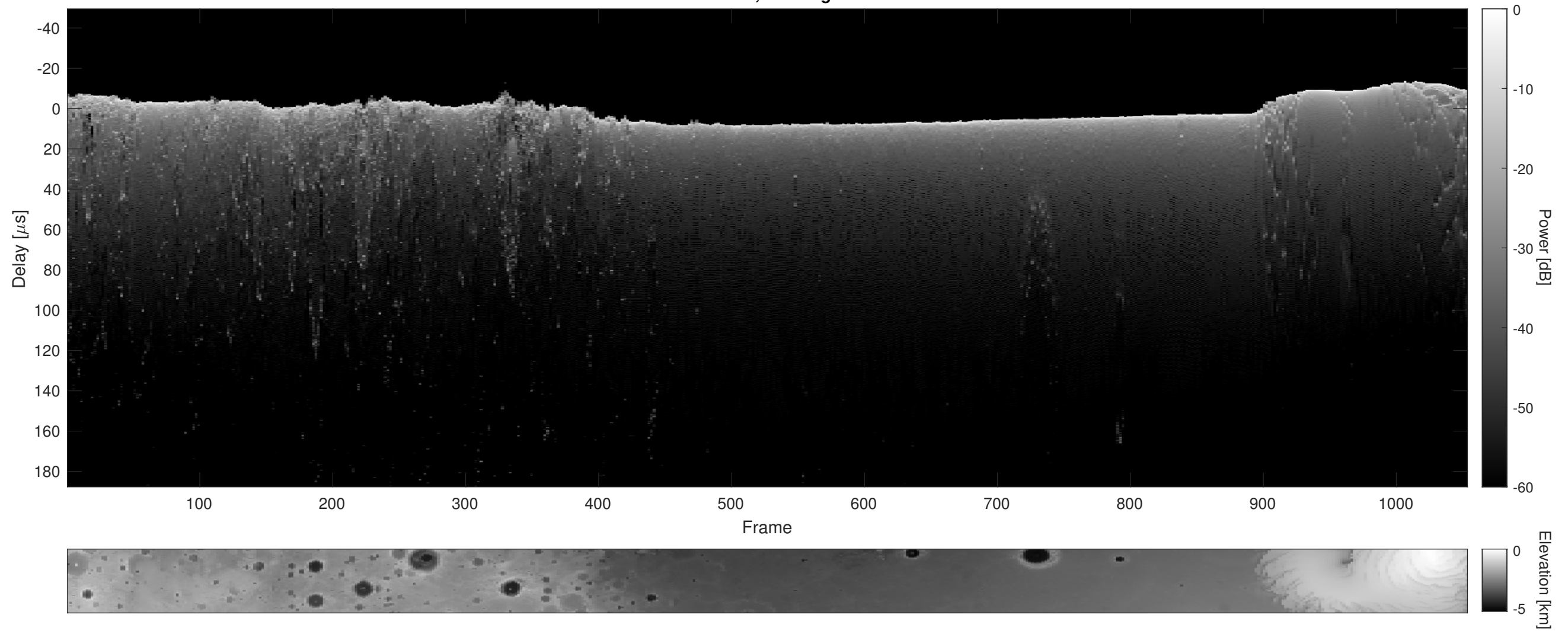
Orbit 7969, Cluttergram
