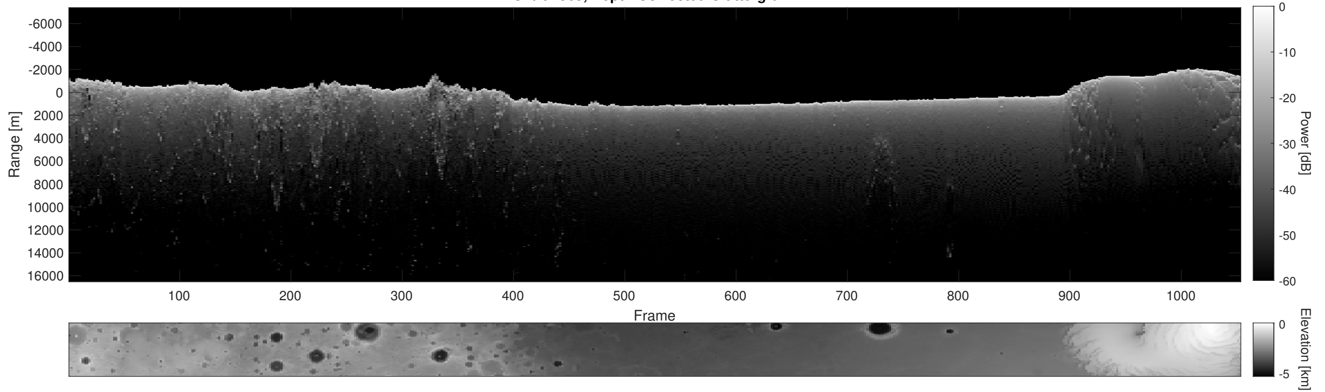
Orbit 7969, Depth-Corrected Cluttergram
