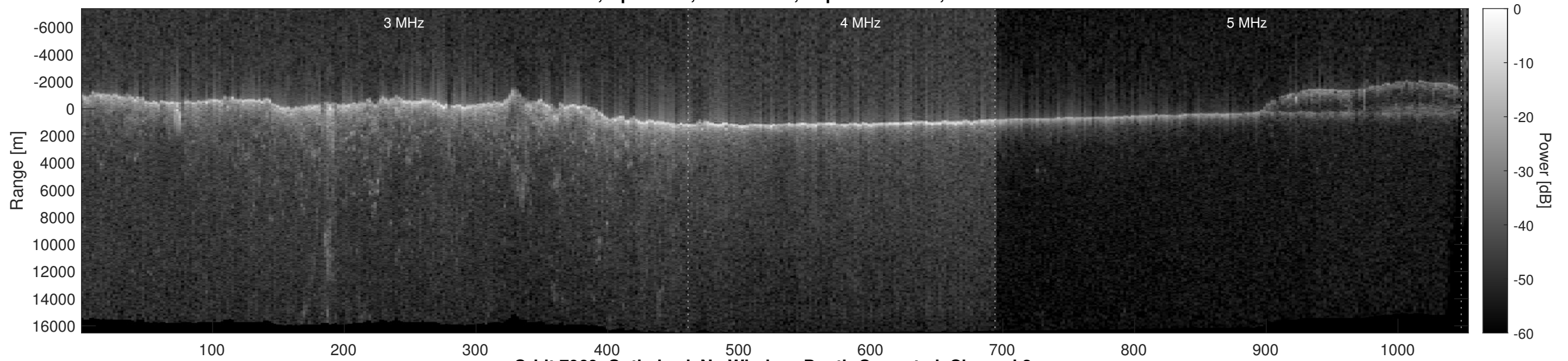
Orbit 7969, Optimized, No Window, Depth-Corrected, Channel 2
