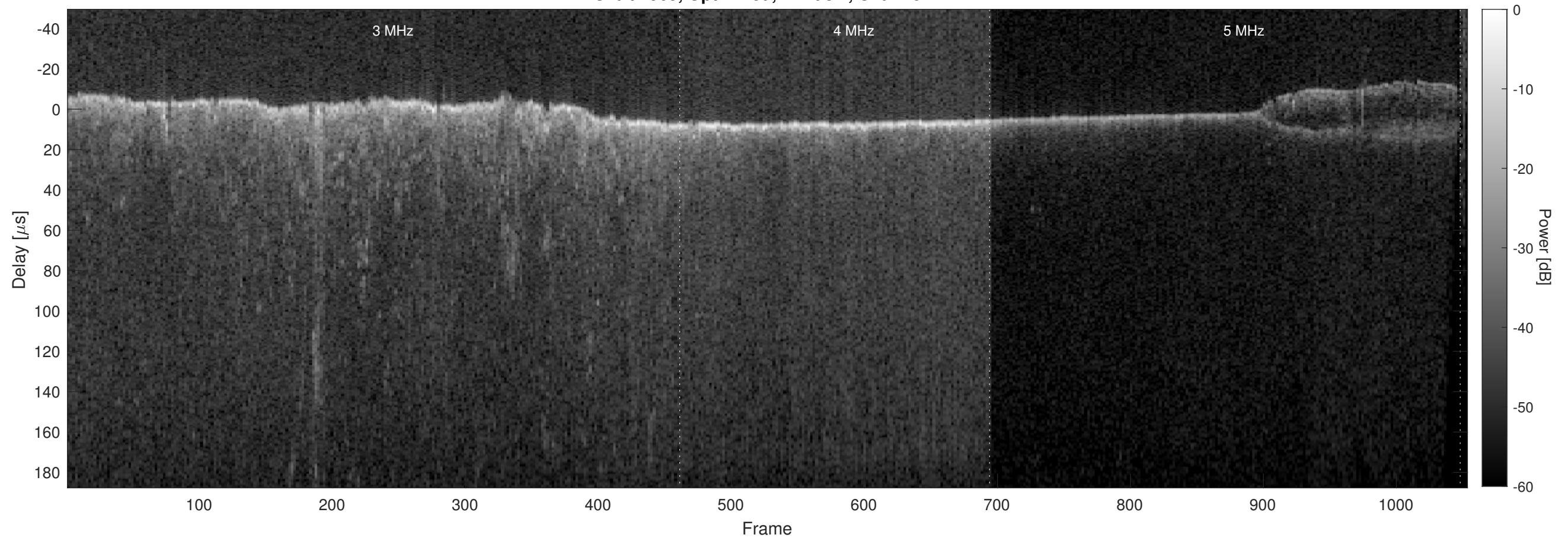
Orbit 7969, Optimized, Window, Channel 2
